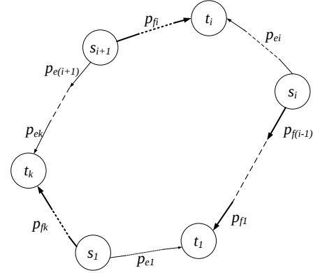
Figure 3: The division of an undirected cycle.
