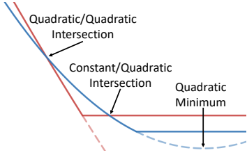
Fig. 5: The set of possible elastic objective intersections.
