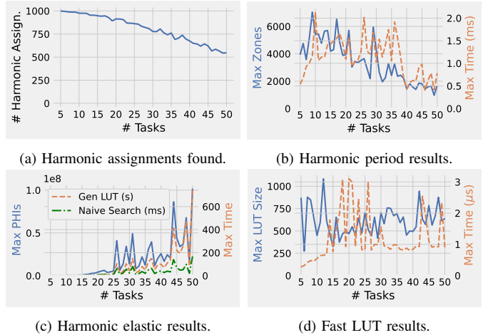
Fig. 8: Evaluation results for synthetic task sets.
