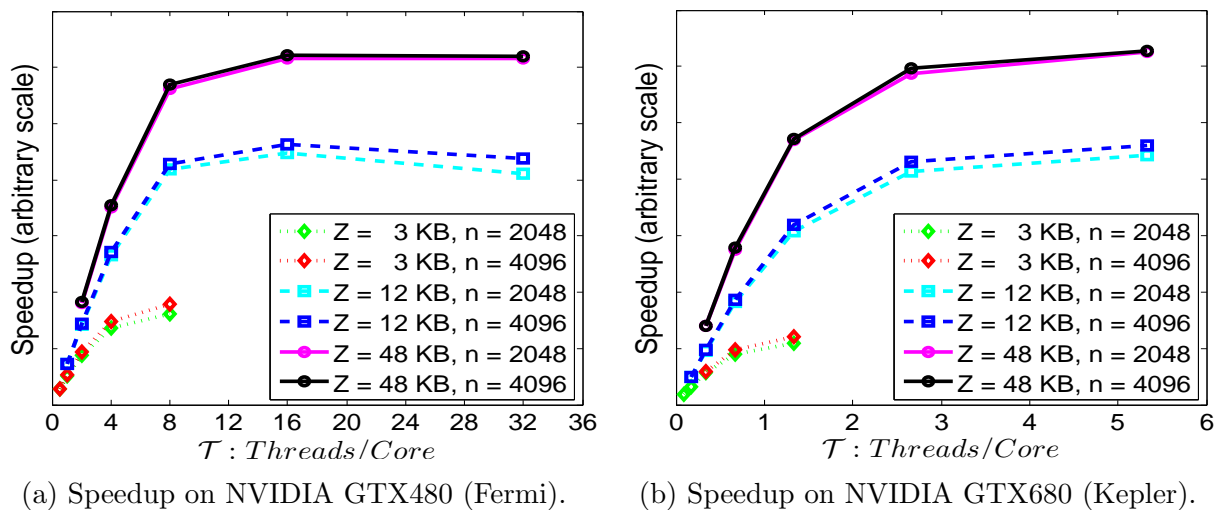
Figure 4.6: Speedup of dynamic programming using adjacency matrix for all-pairs shortest paths problem on two generations of NVIDIA GPUs. On GTX480, with memory size 12 KB and 48 KB, using more than 16 threads hides the memory latency completely; on GTX680, due to the hardware limit on \mathcal{T} , latencies are not fully hidden, and the speedup curve is still climbing slowly.
