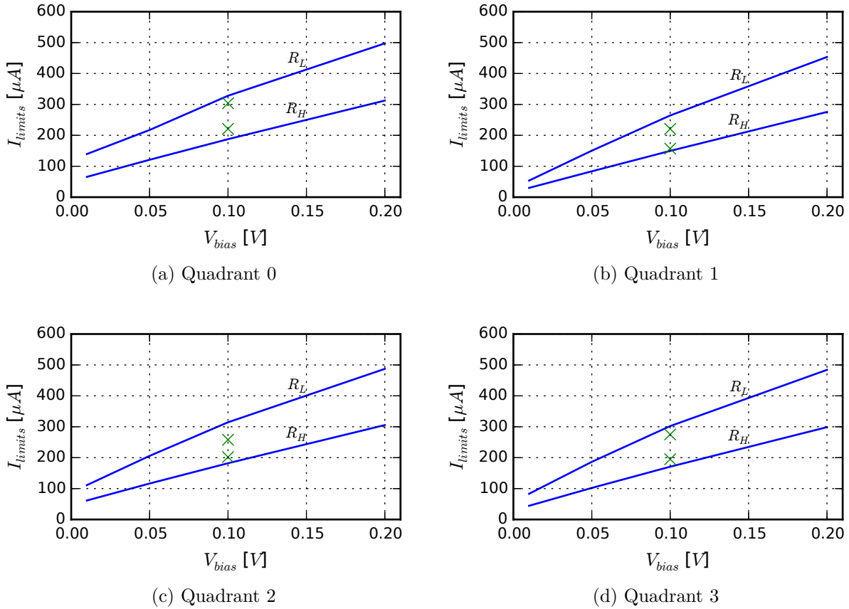
Figure 4.16: Dynamic stability plots showing the stable region of I_{th} currents. These plots show all four quadrants using internal resistors with nominal values R_L = 500 \Omega and R_H = 1 \text{ k}\Omega . The lines are the ideal current limits for a theoretical current comparator. The green \times 's are the measured current limits of the stable range for the actual current comparator in the dynamic test.
