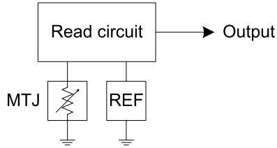
Figure 2.2: Read circuit block diagram for an MTJ. The read circuit senses an MTJ resistance and compares this to a reference to produce an output.
